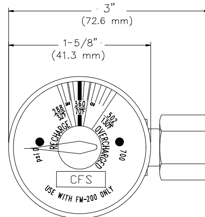
Pressure Gauge
