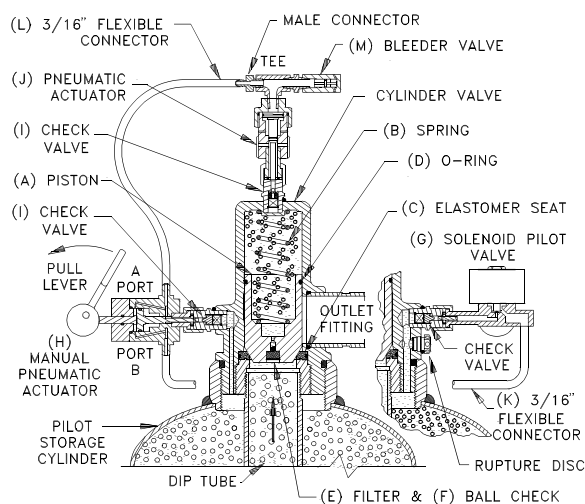
Cylinder Valve - Standby Mode
