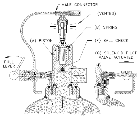
Cylinder Valve - Actuated Mode
